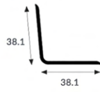
1.5° INTERNAL ANGLE *
