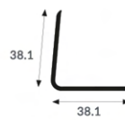
1.5° EXTERNAL ANGLE *
