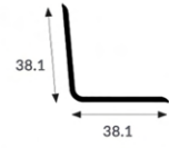
1.5° INTERNAL ANGLE
